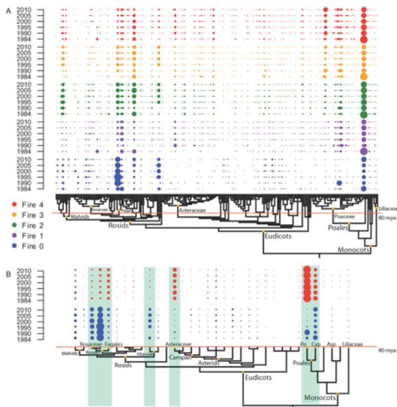
Figure 8. The influence of prescribed burning and the 1988 drought on phylogenetic beta diversity in the oak savanna burn experiment from 1984-2010. Circle sizes are proportional to relative abundance. Frequently burned communities (red) had the highest species richness, the most resource-conservative leaf traits, and spanned the greatest number of lineages, but had more close relatives within lineages. Unburned communities (blue) had the lowest diversity and the fewest lineages, but close relatives co-occurred less frequently. Phylogenetic turnover between treatments is greatest ~80 million years ago (red line). (Cavender-Bares & Reich, in press)
