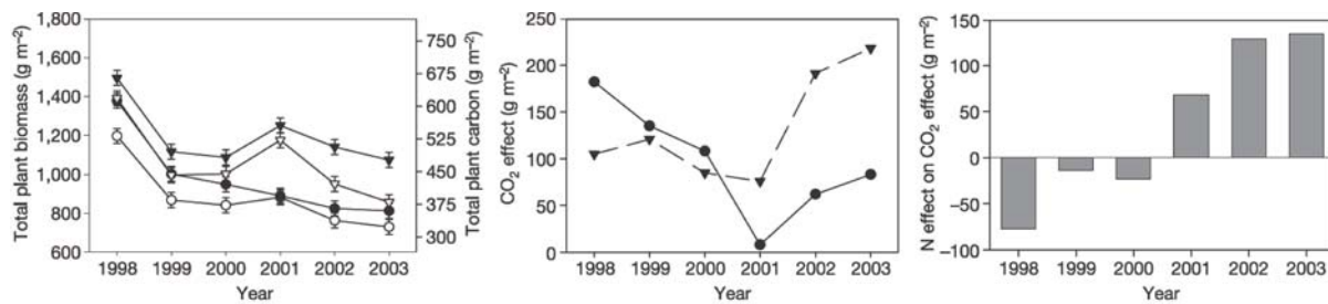
Figure 5. The constraining effect of N limitation on the response of total plant biomass to CO 2 over time in E141. (a) Annual mean total plant biomass (above-ground plus 0–20 cm below-ground) and carbon at ambient CO 2 and N (open circles), elevated CO 2 and ambient N (filled circles), ambient CO 2 and enriched N (open triangles), and elevated CO 2 and enriched N (closed triangles), pooled across diversity treatments. (b) The annual effect of CO 2 on total plant biomass (elevated CO 2 biomass - ambient CO 2 biomass) under ambient N (circles) and enriched N (triangles). (c) The annual effect of N availability on the CO 2 biomass effect (triangle – circle). (Reich et al. 2006)
