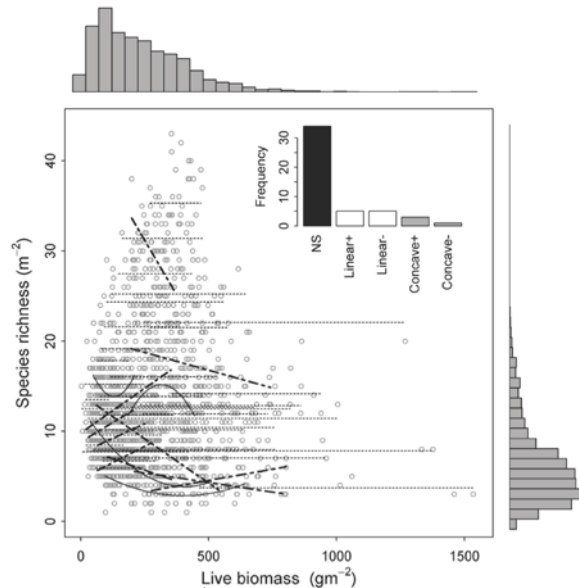
Figure 9. Within-site dependence of plant diversity on productivity (peak live biomass dry weight) across NutNet sites, including the CDR NutNet site. The inset shows the frequencies of relationships that were non-significant (thin dashed lines), linear (thick dashed lines), or concave-up or -down (solid curves). The marginal histograms show the frequency of species richness and peak live biomass across all sites. No “hump shaped” dependence of local diversity on productivity was found within sites, within regions, or across the globe. (Adler et al. 2011)
