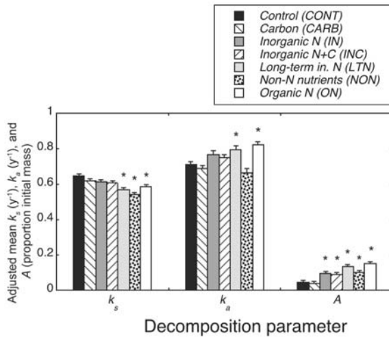
Figure 2. Adjusted mean decomposition parameters from fits of single exponential and asymptotic models to data that show faster initial decomposition rates ( k_s ), but larger slowly decomposing pools ( A ) in treatments that include N addition (IN, INC, LTN, ON) in E211. k_s , single-exponential model decomposition rate; k_a , asymptotic model decomposition rate; A , asymptote. Values are adjusted treatment means with SE bars. Asterisks indicate significant Bonferroni-corrected pairwise comparisons within a decomposition parameter of all treatments with the control. (Hobbie et al. in revision)
