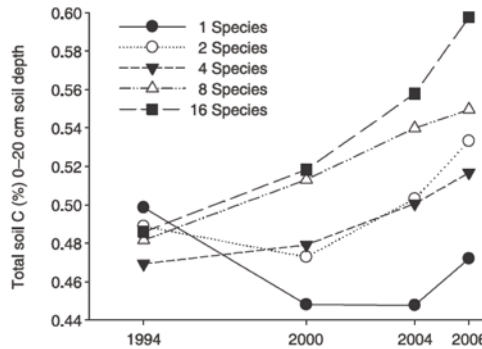
Figure 13. Soil C dynamics in BigBio. During the 12-year period analyzed, soil C declined in monoculture plots but increased at higher diversity, with the greatest increase in 16 species plots. (Fornara and Tilman, 2008)
