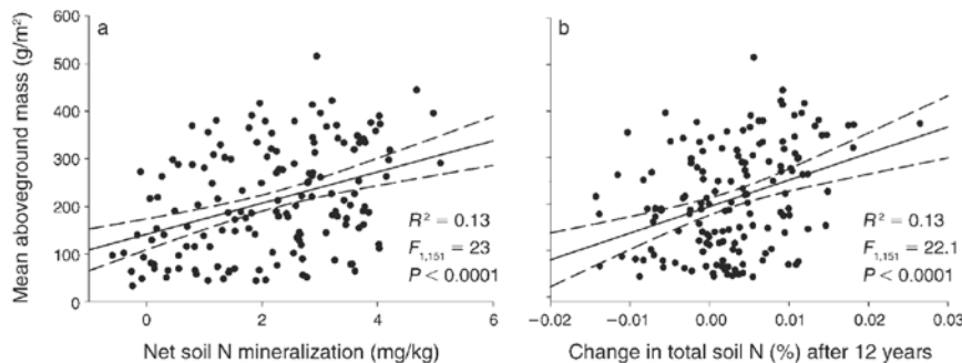
Figure 19. Plant diversity treatments caused changes in soil total C and N content, and in N mineralization rates (Fornara and Tilman 2009). Plant productivity was significantly positively correlated with (a) N mineralization and (b) the change in total soil N over the first 12 years of the BigBio experiment.
