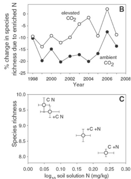
Figure 7. (b) Mean change in species richness ( \pm SE) with added N in elevated and ambient CO 2 and (c) relationship between soil solution N (0–20 cm) ( \pm SE) and species richness under ambient and enriched CO 2 and N treatments in BioCON. Elevated CO 2 reduces losses of plant diversity caused by N deposition. (Reich 2006)
