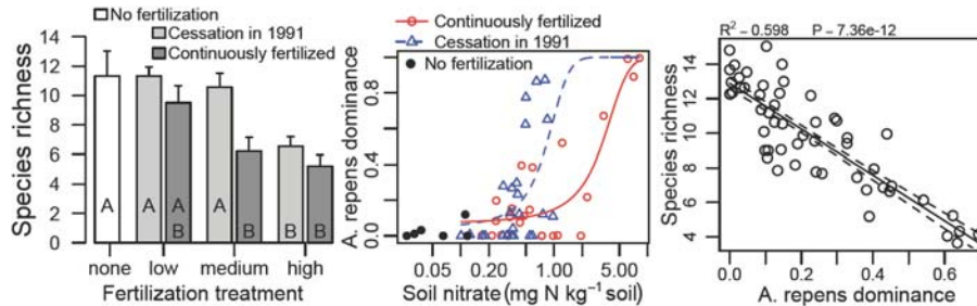
Figure 17. (a) Species richness (number of species 0.3 \text{ m}^2 ) versus N addition in 2011. While some plots received continuous N addition (1982-2011; dark gray bars), N addition was ceased in 1991 in other plots (light gray). After three decades, plots were either species rich (no N addition, or cessation of low and medium rates of N addition) or species poor (high N addition and cessation of high N addition). Treatments significantly differed (ANOVA; F_{6,47}=7.38 , P<0.0001 ); different letters indicate P<0.05 for Tukey contrasts. (b) Agropyron repens , an exotic perennial, exhibited hysteresis as it shifted between these rarity or abundance in response to changes in soil nitrate (in \log_{10} scale). (c) High abundance of Agropyron repens was associated with low diversity of native plant species. (Isbell et al., in prep)
