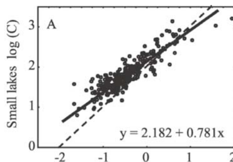
Figure 23. Scale dependent stoichiometry in small lakes from around the world. As indicated by the slope less than one, seston stoichiometry at the whole small-lake scale (dots, n = 281 lakes) deviates significantly from the Redfield 106:1 proportionality (dashed line), which is a good representation of the relationship between seston C and seston P at larger observational scale, taking in multiple aquatic habitats including fresh and saline waters. Similar differences in the coupling of elements across scales are seen with other element ratios and in other habitats in fresh and saline waters, a difference which has been hypothesized to result from the inclusion of greater environmental heterogeneity. (Sternner 2008; Sternner et al. 2008)
