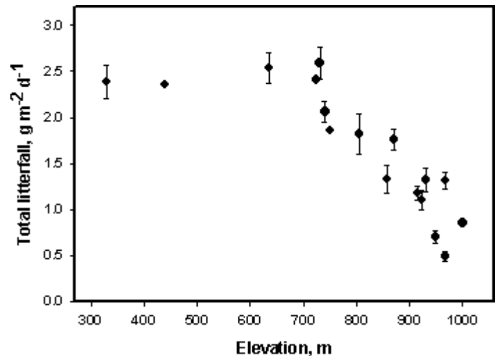
Fig. 2.5.4. Aboveground litter production as a function of elevation in the LEF. Data are from Weaver and Murphy (1986), Scatena et al. (1996), and Silver et al. (in prep.).
