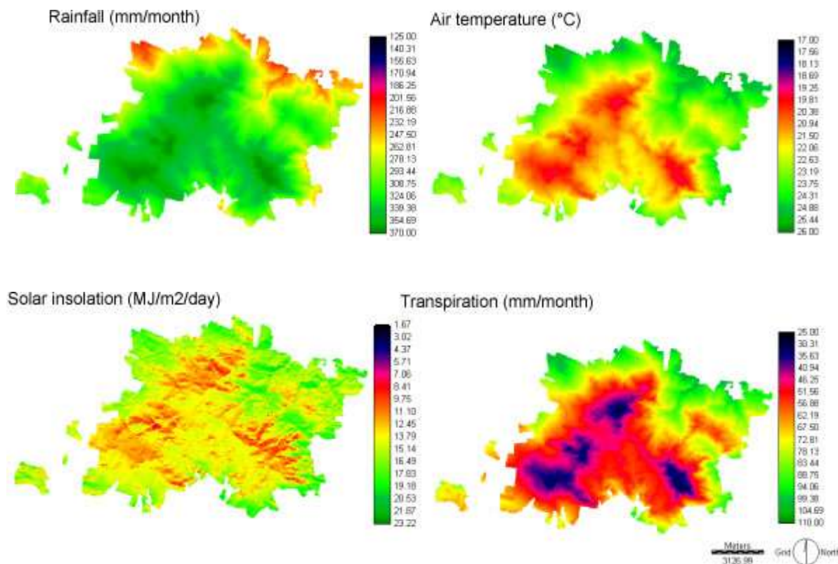
Fig. 2.5.1. Climate variation in the Luquillo Experimental Forest as depicted in the L-CENTURY model (from Wang 2001). Note that less intense colors represent higher values.
