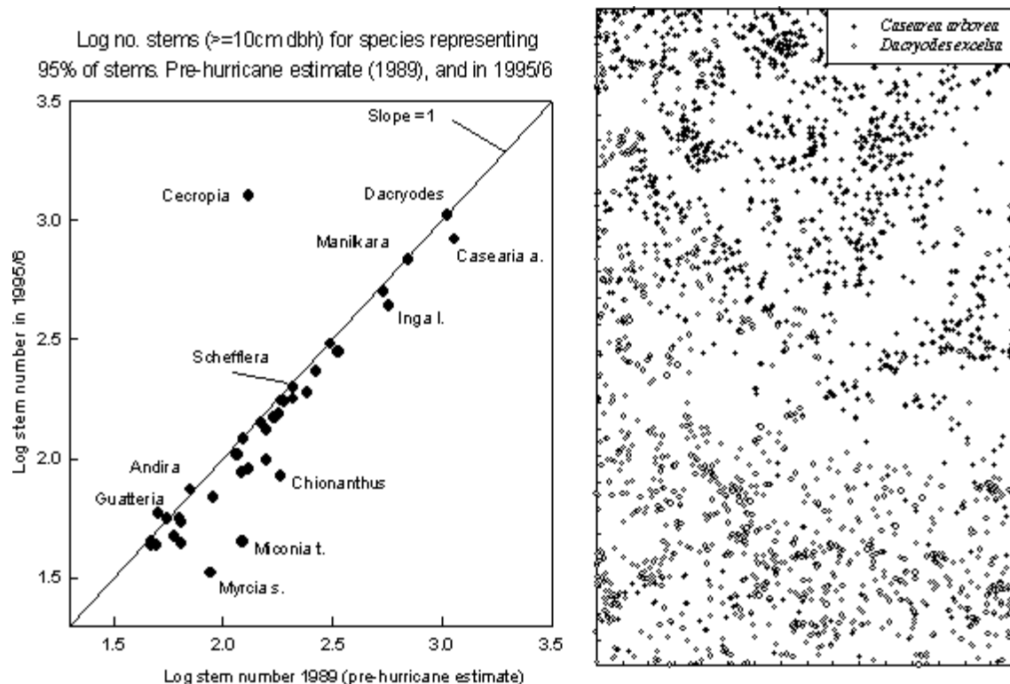
Fig. 2.3.4. Results from the 16-ha Luquillo Forest Dynamics Plot showing (lefthand graph) the stability of species composition in response to Hurricane Hugo (1989). Note the exceptional increase
