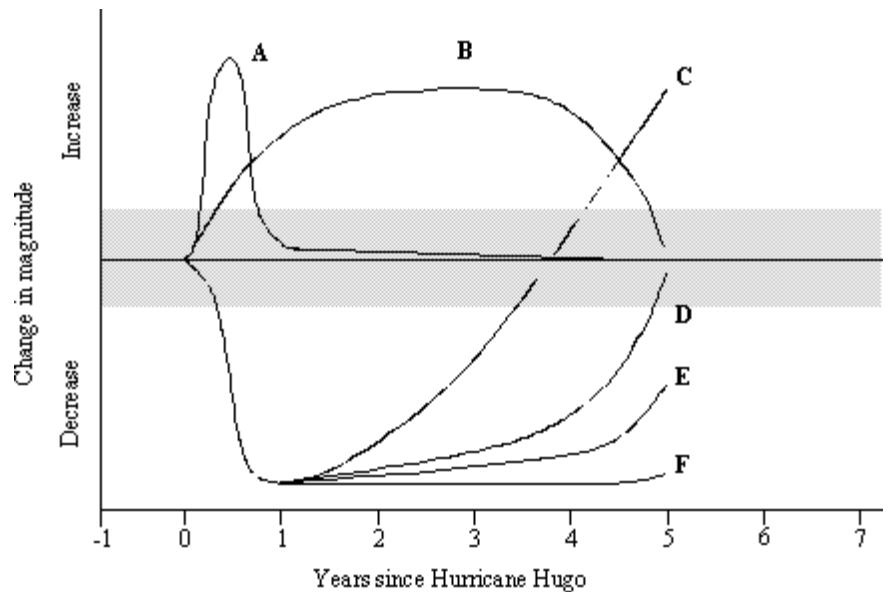
Fig. 2.4.1. Idealized 5 yr trajectories of responses of different components of wet subtropical forest in the Luquillo Experimental Forest, Puerto Rico, to disturbance caused by Hurricane Hugo (from Zimmerman et al. 1996). The shaded portion of the graph represents \pm 15 percent variation indistinguishable from pre-hurricane values. Curve A: transient ( <1 yr) increase. Examples include forest floor biomass, some soil nutrient pools, and nitrate concentrations in streams. Curve B: slow increase and return to pre-hurricane levels. Examples are net primary productivity, abundance of Atya shrimp in streams, of adult coqui frogs, and of the terrestrial snail, Cepolis squamosa . Curve C: catastrophic decrease and subsequent rise above pre-hurricane levels. Examples are aboveground pools of potassium and magnesium and of several species of terrestrial snails. Curve D: catastrophic decrease and return to near pre-hurricane levels. Examples are tree biomass and tree density. Curve E: a catastrophic decline and steady increase, but not to within 15 percent of pre-hurricane levels. An example is fine total litterfall. Curve F: catastrophic decline and little recovery until 5 yr post-hurricane. Examples are fine root biomass and abundance of the walking stick, Lamponius portoricensis . Both of the latter returned to near normal values subsequently.
