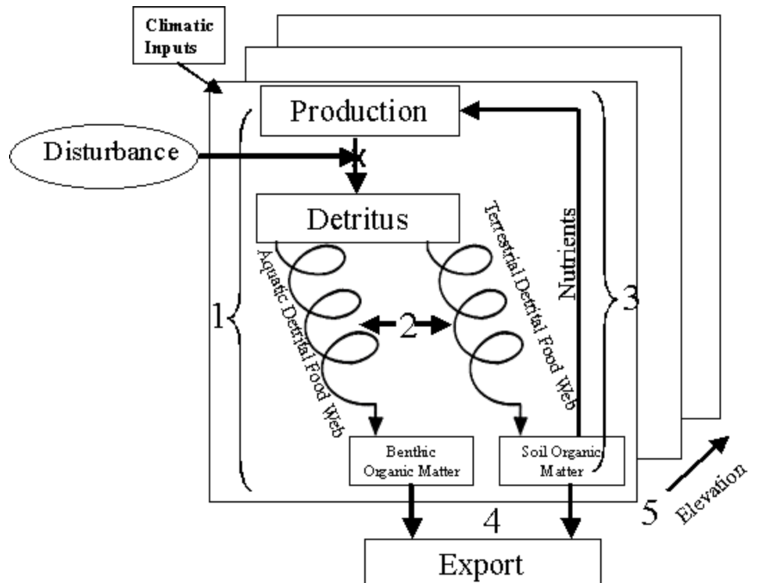
Fig. 2.7.1. Schematic representation of the scientific questions addressed by LUQ during LTER 3: 1) How do climatic factors, litter quality, and detritivore diversity regulate decomposition of detrital pulses? 2) How do terrestrial and aquatic food webs differ in their response to detrital pulses? 3) What is the effect of disturbance frequency on nutrient cycling plant community composition, and the accumulation of soil organic matter? 4) To what degree is the export of carbon and nutrients from watersheds a result of soil characteristics that are affected by detrital dynamics? 5) How do elevationally related changes in climate impact plant and detritivore communities, and how do these feed back on the quantity and quality of litter inputs and decomposition?
