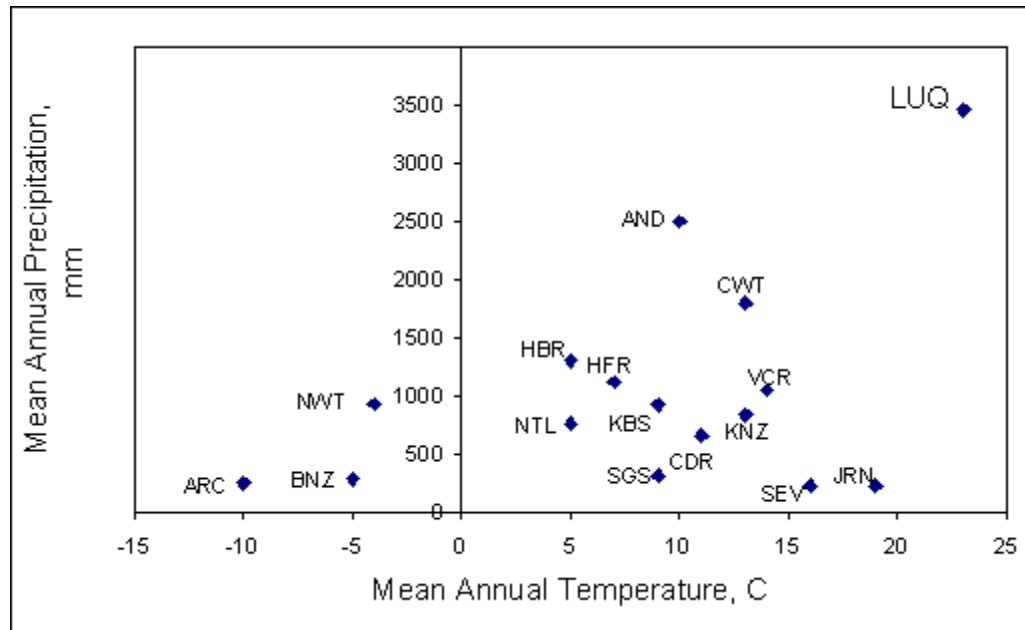
Fig. 2.1.3. Mean annual temperature and precipitation of the Luquillo Experimental Forest relative to other US-LTER sites in the Long-term Intersite Decomposition Experiment. As a result of higher rainfall and temperatures, decomposition in the LEF takes less time than in any of the other US-LTER sites (Gholz et al. 2000).
