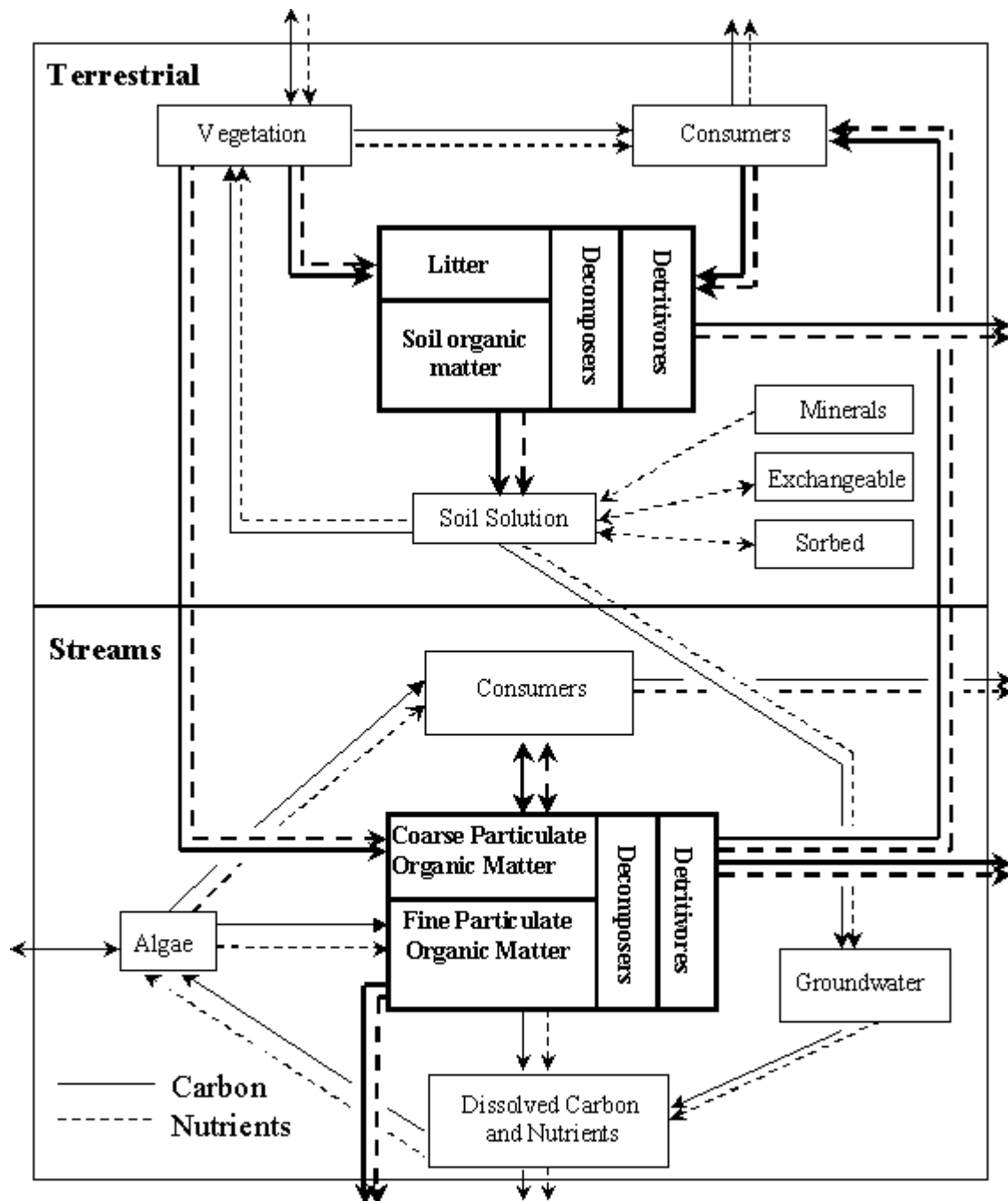
Fig. 2.1.2. A generalized box model of material flow in terrestrial and aquatic ecosystems in the Luquillo Experimental Forest. Compartments and arrows in bold indicate major pools and fluxes of carbon and nutrients associated with detrital dynamics.
