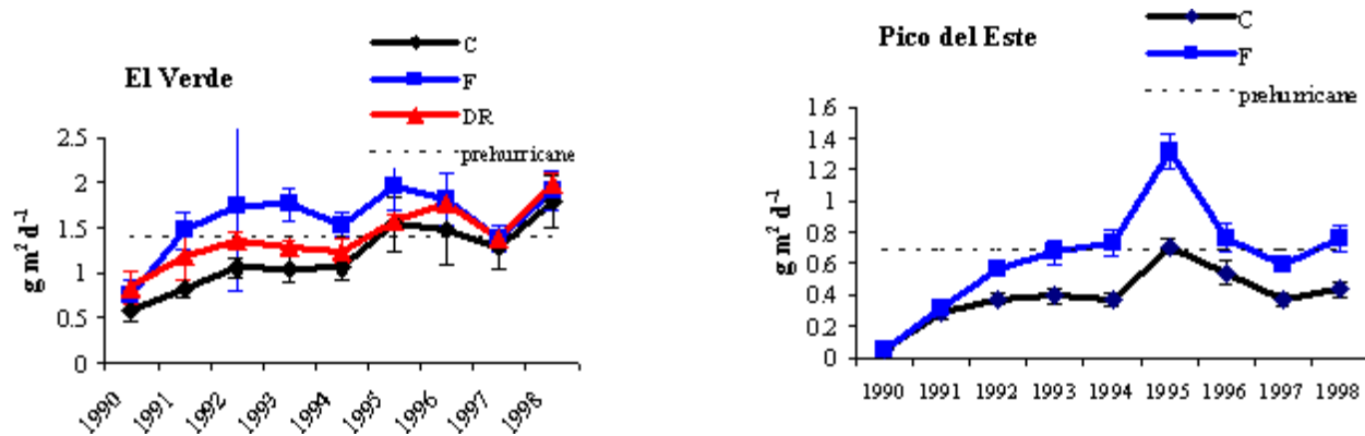
Fig. 2.5.2. Comparison of leaf litter production in (a) mid-elevation (400 m; El Verde) and (b) high elevation (1000 m; Pico del Este) forest plots (Walker et al. 1996, Warren et al. unpublished). The studies began within one year of Hurricane Hugo and show the effect of quarterly fertilization (F: NPK + micronutrients) compared to unmanipulated plots (C). At El Verde, a one-time removal of hurricane generated debris (DR) was also studied (Zimmerman et al. 1995). At El Verde, litter production returned to pre-hurricane levels within seven years of the storm while at Pico del Este this has yet to occur (except during one unusual year). Plots at El Verde also responded more quickly to the addition of supplemental nutrients.
